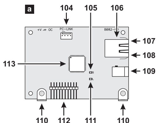
Figura 7 Parti del Modulo IP ABS-IP (a) e del Bridge WiFi ABS-VAP11N (b).
